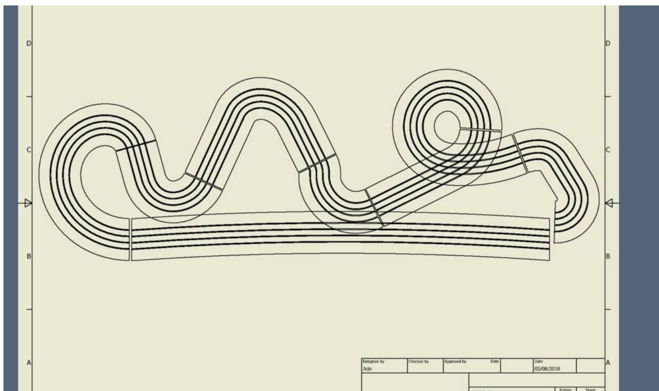
Illustration 18: Conception CAO 3D piste bois Cirso32 (projection verticale) [GSR_15]
